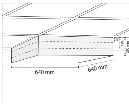
For ceiling 625x625
